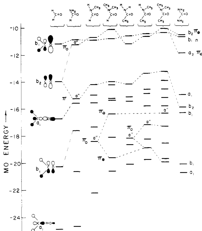
Figure 3. MO energies, as obtained by a CNDO/s computational scheme, for various amides. The upper \pi_O MO (or, in urea, MO's) refers to a \pi MO heavily localized on the amidic nitrogen. The bottom set of MO's refer to \pi MO's which are largely "methyl group" in character; the type of methyl group (i.e., N -methyl or O -methyl) can be decided by inspection of the figure. The geometric parameters chosen were those for the gaseous molecules, 21 except for urea, for which X-ray crystallographic data 22 were used. Computations followed the Del Bene-Jaffé routine. 23 The amides ( C_s symmetry) are correlated with formaldehyde and urea ( C_{2v} symmetry).
