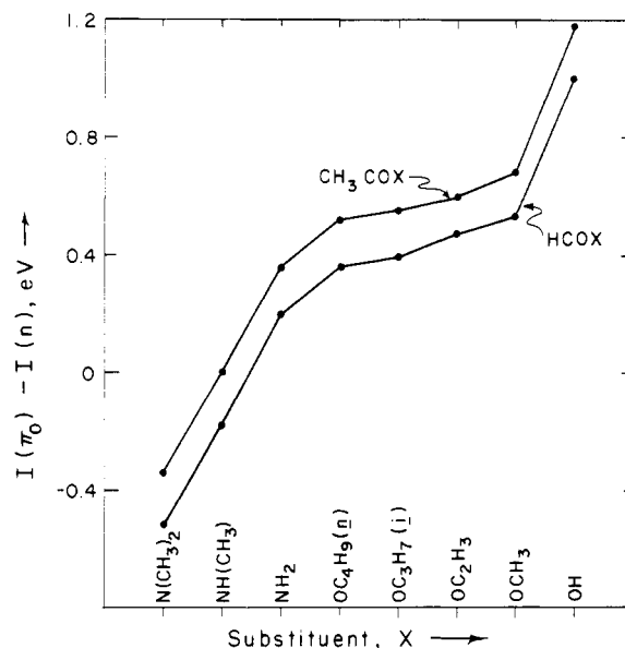
Figure 4. A plot of I(\pi_O) - I(n) for various \text{HCOX} and \text{CH}_3\text{COX} molecules.
